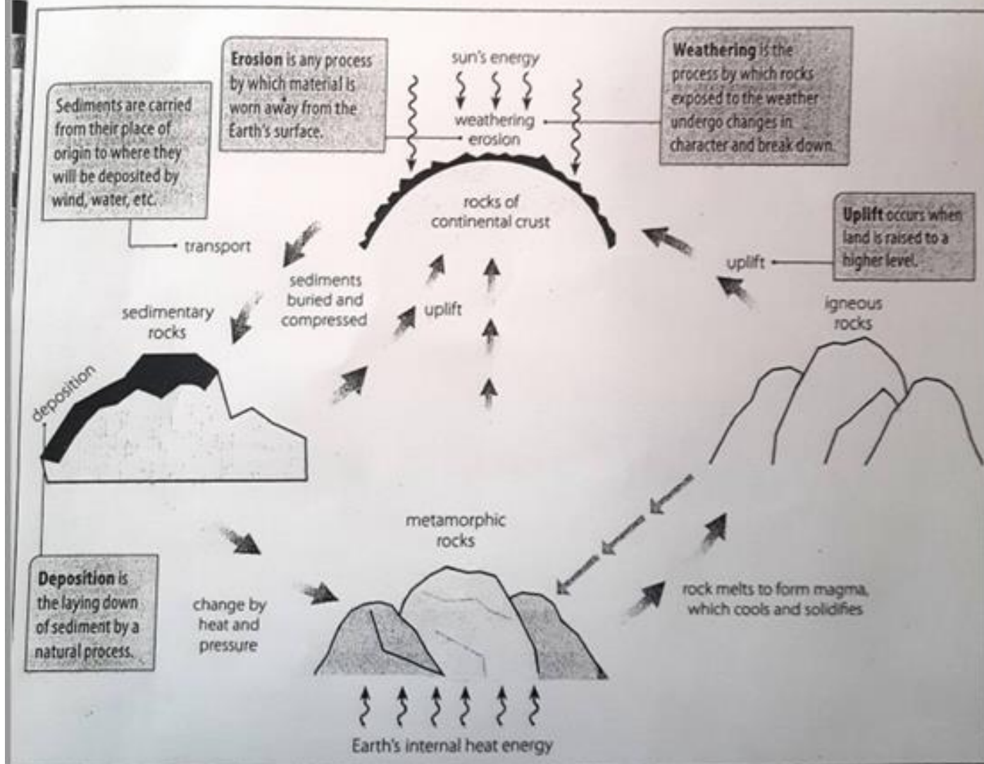
Figure 3.5 The formation of igneous, sedimentary and metamorphic rock
